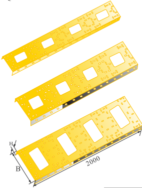
XQJ-ZH-01A 型组合式桥架 Model XQJ-ZH-01A combined Cable Support
