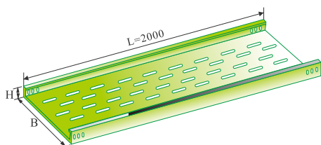
XQJ-P-01托盘直通 XQJ-P-01Tray type straight supply
