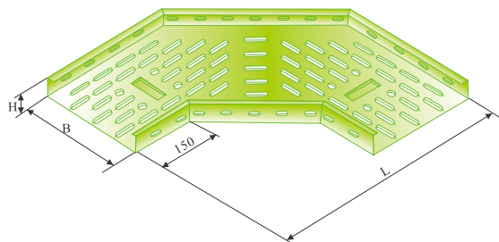
XQJ-P-02水平弯通 XQJ-P-02Tray type horizontal bend
