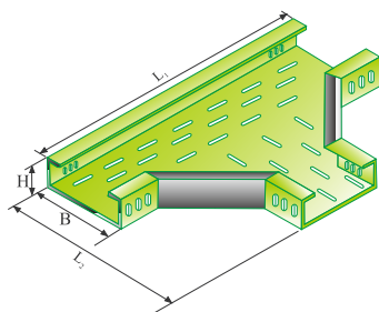
XQJ-P-03水平三通 XQJ-P-03Tray type horizontal Tee
