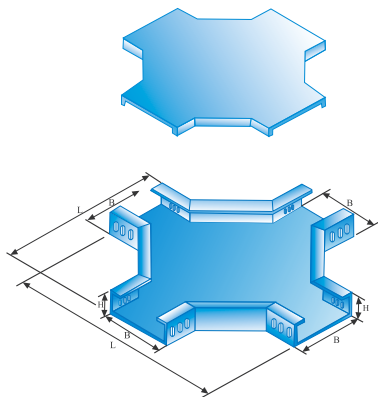
XQJ-C-4A水平四通 XQJ-C-4AHorizontal 4-Way
